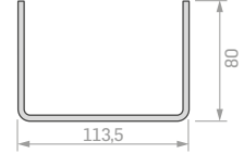
• 1745 Kare Kolon İçi U Profil SQUARE COLUMN INSIDE U PROFILE Ağırlık / Weight: 2,821
